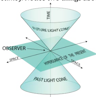
Figure 1. Hypothetical Minkowski 4-D Spacetime
