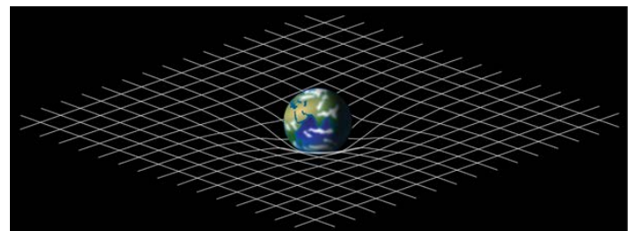
Figure 2. Hypothetical Fabric of Spacetime
